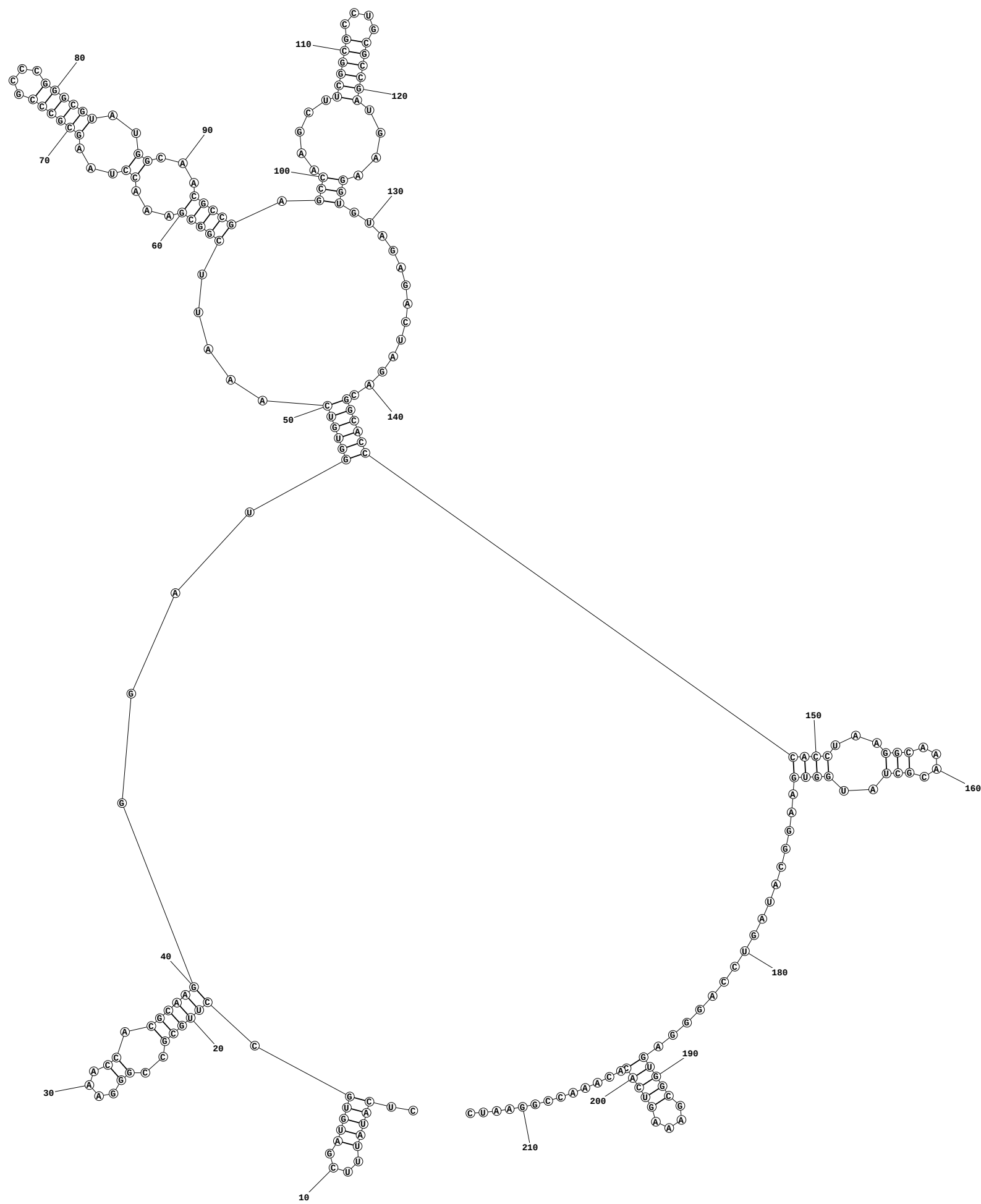
Group_I_intron_Azoarcus_sp
