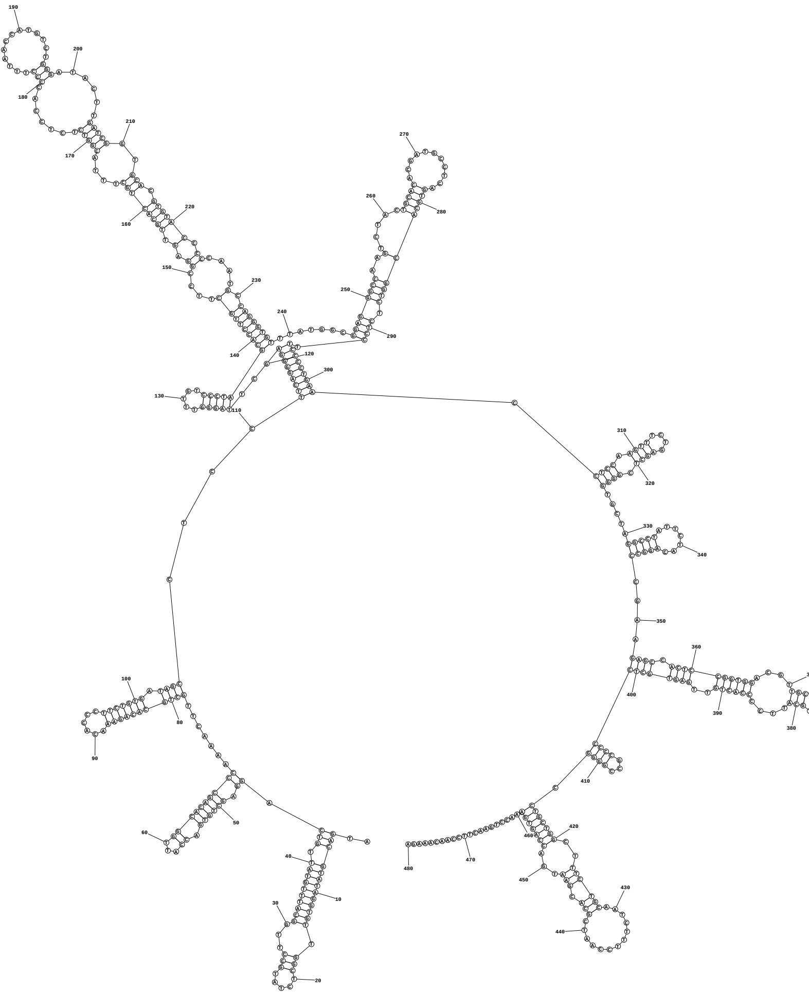
seq1_predicted
